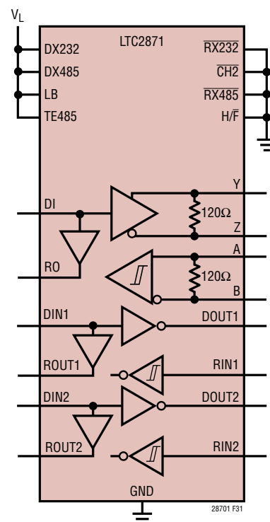
Figure 32. LTC2871 in RS485 and RS232 Mode with Loopback and RS485 Termination
