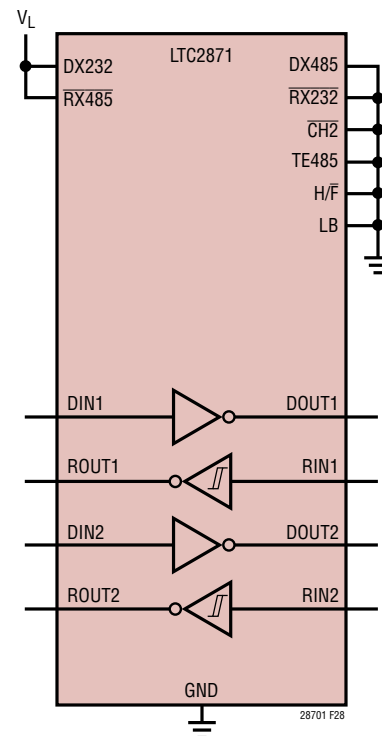
Figure 29. LTC2871 in RS232 Mode
