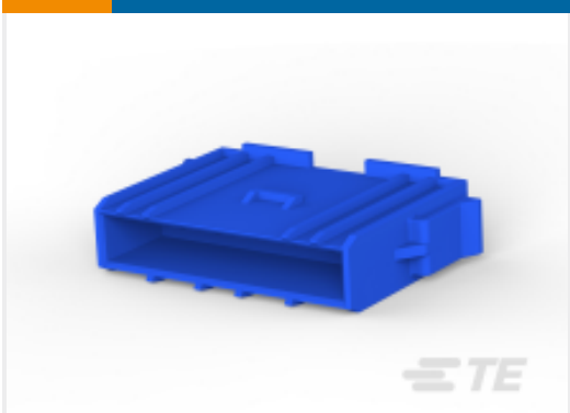
TE Part #2120050-1 FF HOUSING 6P NYLON BLUE
