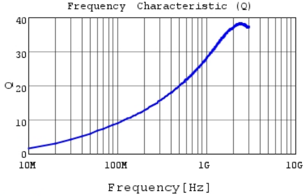
LQP03TN5N6H02 Q
