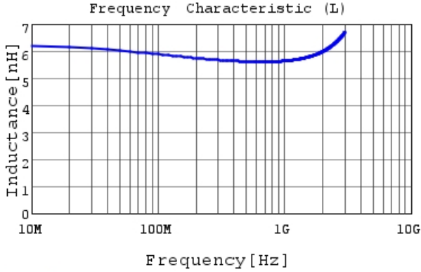
LQP03TN5N6H02 L
